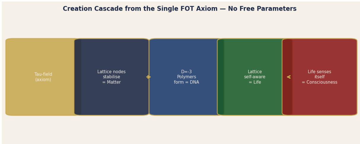
Figure 4. Creation cascade from the single FOT axiom. Five steps from Tau-field (axiom) through matter, DNA, life to consciousness. Each step is a register depth transition with no additional parameters.
